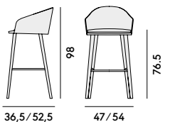
057 Sgabello in frassino, con sedile imbottito / Barstool in ashwood, with upholstered seat
